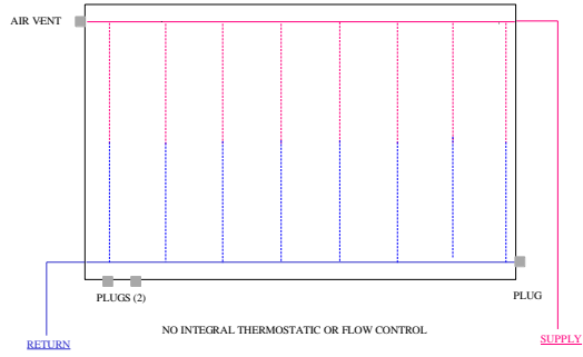
PENSOTTI PANEL RADIATORS - ALTERNATE PIPING ARRANGEMENT 2
