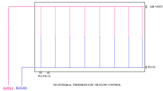
PENSOTTI PANEL RADIATORS - ALTERNATE PIPING ARRANGEMENT 5
