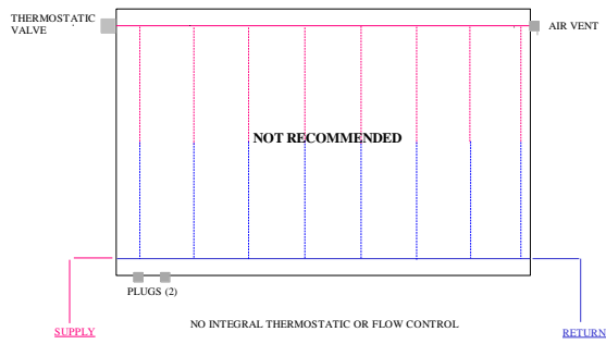
PENSOTTI PANEL RADIATORS - ALTERNATE PIPING ARRANGEMENT 3
