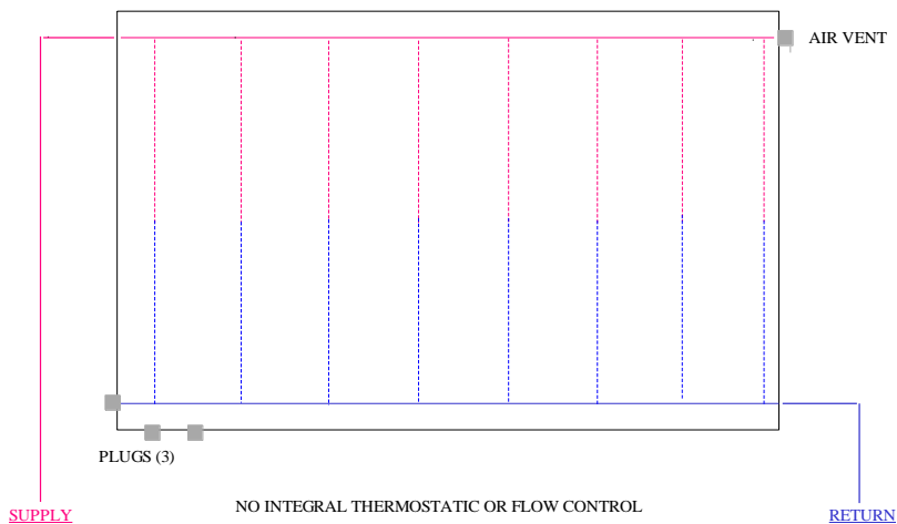
PENSOTTI PANEL RADIATORS - ALTERNATE PIPING ARRANGMENT 1
