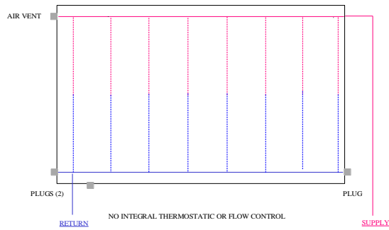
PENSOTTI PANEL RADIATORS - ALTERNATE PIPING ARRANGEMENT 3
