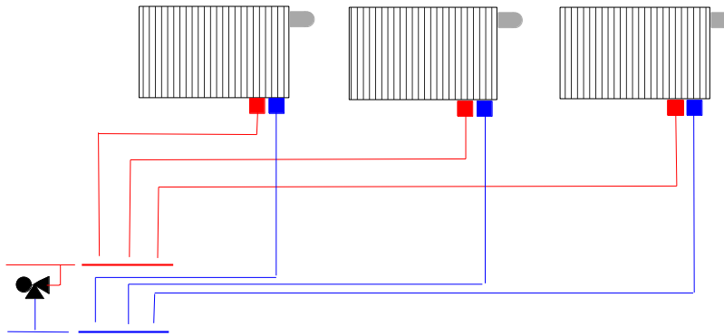
Homerun with Thermostatic Operators and By-Pass Valve
