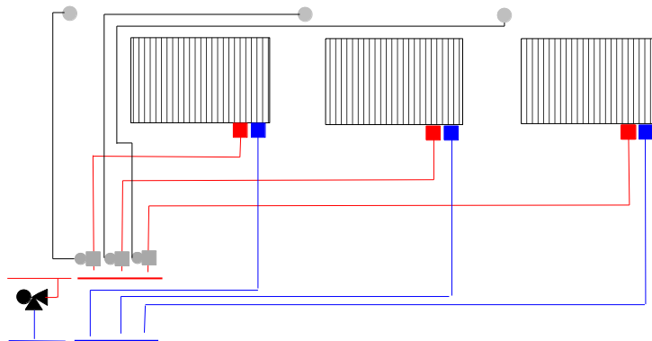
Homerun with Electric Zone Valve and By-Pass Valve
