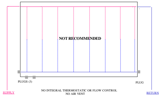
PENSOTTI PANEL RADIATORS - ALTERNATE PIPING ARRANGEMENT 7
