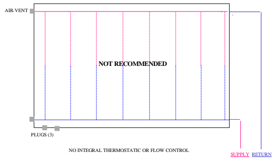
PENSOTTI PANEL RADIATORS - ALTERNATE PIPING ARRANGEMENT 4
