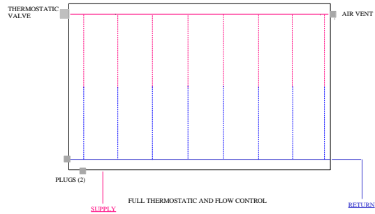
PENSOTTI PANEL RADIATORS - ALTERNATE PIPING ARRANGEMENT 4
